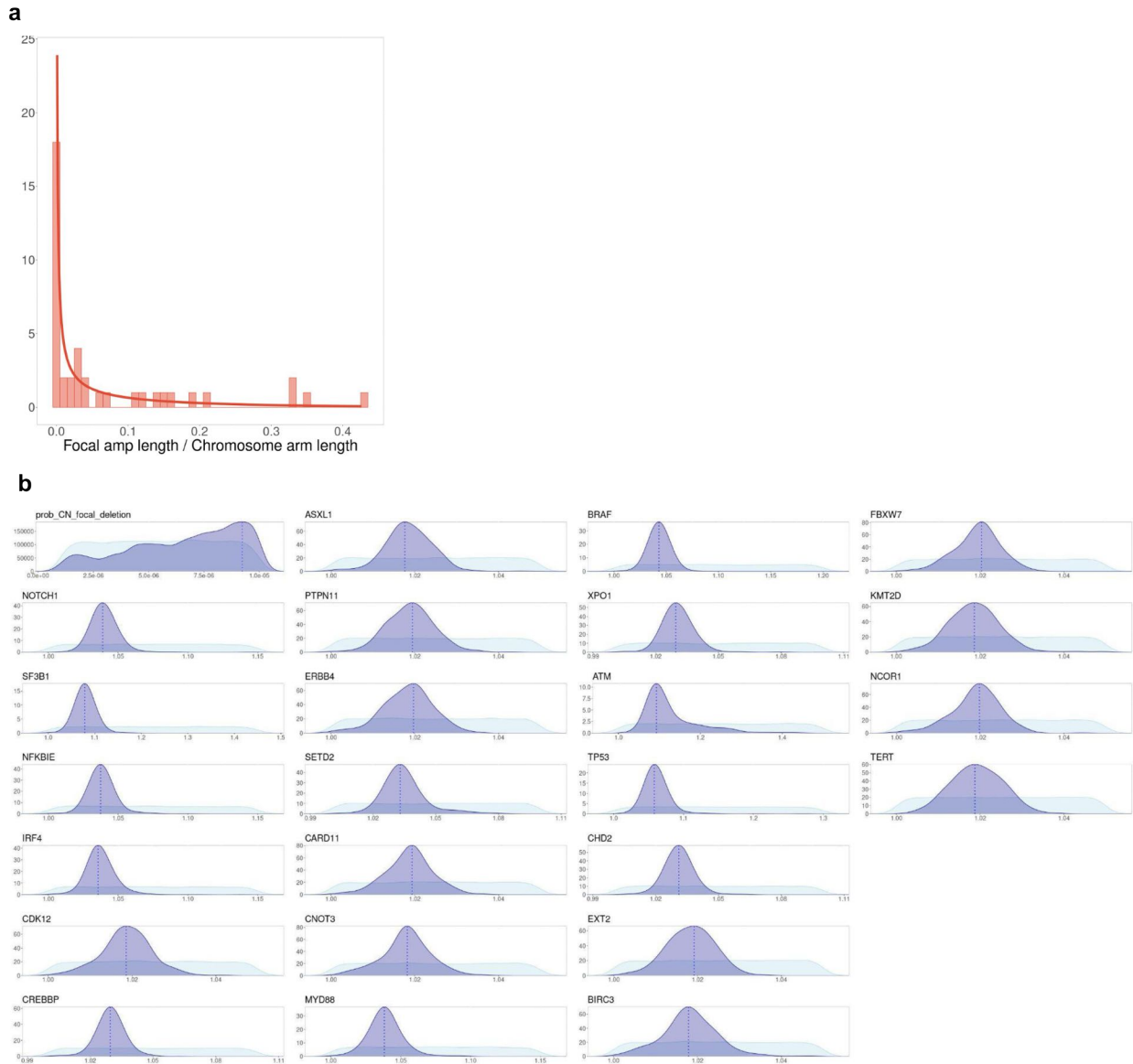
Supplementary Figure 24. Inference of driver gene selection rates in CLL-ES (PCAWG). (a) Ratios of focal amplification lengths over corresponding chromosome arm lengths are fitted with a Beta distribution. (b) Prior distribution (light blue) and posterior distribution (dark blue) from inference with ABC random forest. Broken line represents the mode in the posterior distribution for each parameter.
