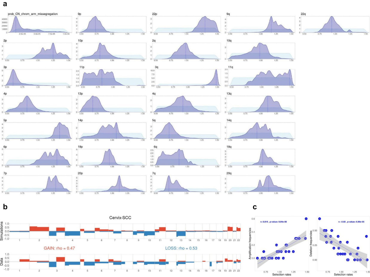
Supplementary Figure 2. Inference of chromosome-arm selection rates in Cervix-SCC (PCAWG). (a) Prior distribution (light blue) and posterior distribution (dark blue) from inference with ABC random forest. Broken line represents the mode in the posterior distribution for each parameter. (b) Comparison between simulations with fitted parameter (top) and gain/loss frequencies at arm level from TCGA (bottom). The simulations are computed with the posterior modes from (a) . Spearman's correlation coefficient \rho between frequencies of gains (or losses) among each arm in PCAWG and simulations. (c) Correlation between inferred selection rates and amplification/deletion frequencies for individual chromosome arms. Linear regressions and p-values from Pearson correlation.
