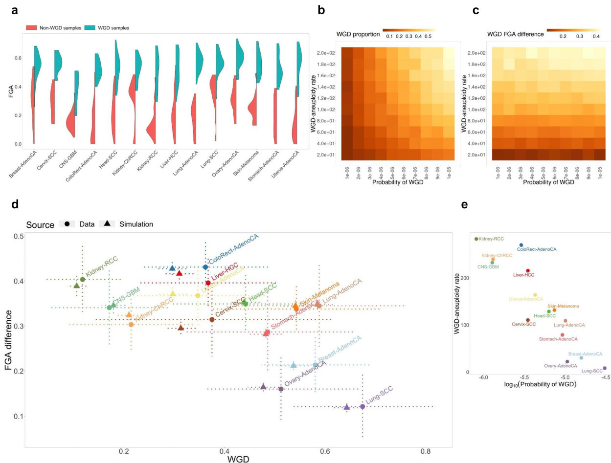
Figure 4. Results from fitting WGD parameters to CN data from PCAWG. (a) Distribution of Fraction of Genome Altered (FGA) in PCAWG by cancer type and WGD status. (b-c) Impact of varying WGD probability and WGD-aneuploidy rate on WGD proportion (b) and WGD FGA difference (c) in simulated samples. WGD FGA difference is defined as \text{mean}(\text{FGA}|\text{WGD}) - \text{mean}(\text{FGA}|\text{non-WGD}) . 1,000 simulations are created for every parameter combination. (d) Comparison between WGD proportion and WGD FGA difference from the fitted model (triangle) and PCAWG (circle). Dotted bars represent ranges of each statistic from 10,000 bootstrap samples. (e) Comparison between inferred WGD probability (in logscale) and WGD-aneuploidy rate for each cancer type.
