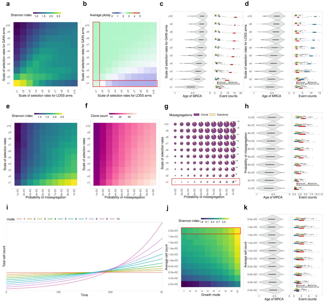
Figure 3. Analysis of parameters in the chromosome arm selection model. (a-b) Effects of selection rates for GAIN and LOSS chromosome arms on average Shannon diversity index (a) and average ploidy in each sample (b) . (c-d) MRCA age and average missegregation counts, grouped based on clonality (clonal/subclonal) and type (gain/loss), as selection rates for GAIN arms (c) or LOSS arms (d) increase (variables correspond to highlighted segments in (b) ). MRCA age is computed as fraction over time back to when simulation starts. MRCA age = -1 if the sampled cell phylogeny tree starts branching at the beginning of the simulation. MRCA age \rightarrow 0 as the MRCA is closer to sampling time. (e-g) Effects of probability of missegregation and chromosome-arm selection rates on average Shannon diversity index (e) , clone count (f) and average count of clonal and subclonal missegregations (g) (size of circles indicates the total missegregation counts). (h) MRCA age and missegregation counts as probability of missegregation increases (variables correspond to highlighted segment in (g) ). (i) Different patterns of growth mode, ranging from constant (mode 1) to exponential with high growth rate (mode 10). (j) Effect of growth mode and average cell count on average Shannon diversity index. (k) MRCA age and missegregation counts as average cell count increases (variables correspond to highlighted segments in (j) ). 1,000 simulations are created for every parameter combination.
